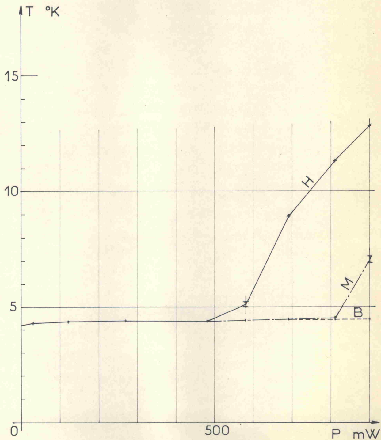
FIG.2 Normal helium T = 4.2 K ; P = 760 mm Hg Depth of immersion : 20 cm
